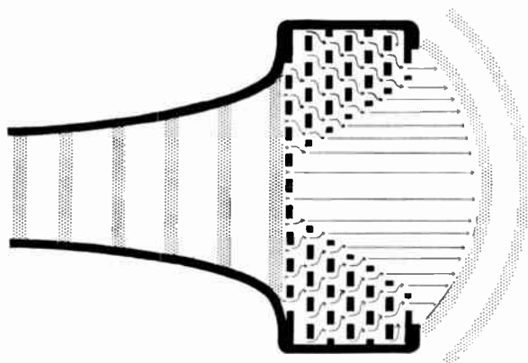
FIG. D/7. Sectional diagram of acoustic lens with perforated plates showing time-lag and wider dispersion.
