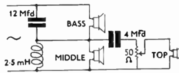
N.W.10. Quarter Section, 3-speaker circuit. Crossover at 1,000 and 5,000 c/s.
