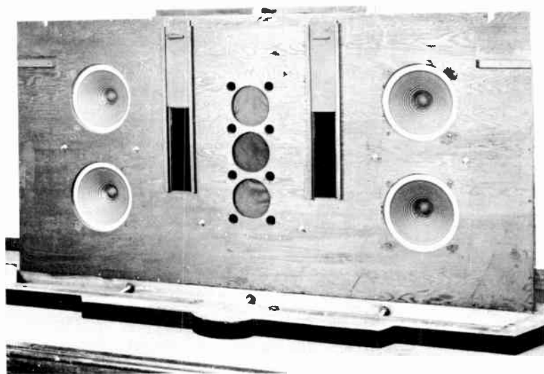
FIG. O/1. Loudspeaker system for electronic organ.
