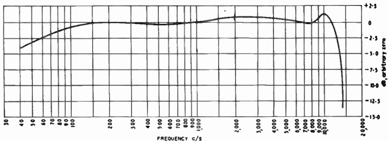
FIG. F/9B. Frequency response of tape recorder used in tests by Mr. Shorter and Mr. Manson.
