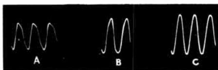
FIG. N/1. Non-linearity at A and B at 40 c/s with 1 watt input to 10" unit. A—Corrugated paper surround. B—Cloth surround. C—Foam plastic surround.
