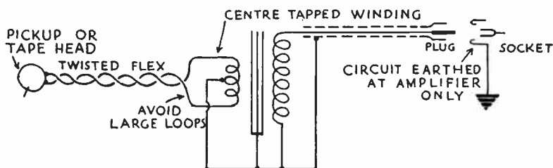
FIG. H/4. Input circuit with centre-tapped transformer arranged to avoid hum.
