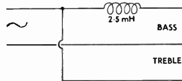
N.W.2. Simple low-pass filter
