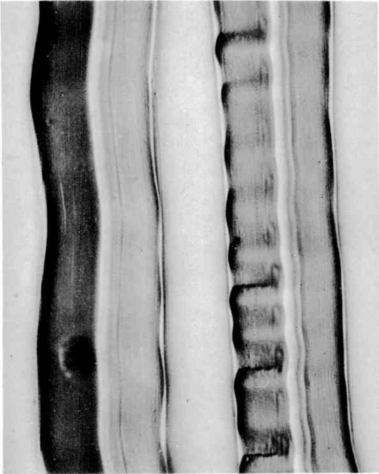
FIG. R/16. Groove after 165 playings showing little wear. Mag. 300x.
