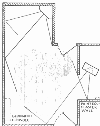
FIG. R/21. Unusual speaker set-up providing good stereo reproduction in the two listening areas which are shaded, and good general reproduction using both speakers with mono input.
