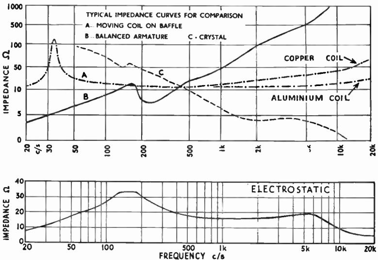
FIG. 1/1. Typical impedance curves.
