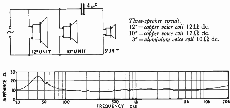
FIG. 1/2. Unusually level impedance curve achieved by parallel working.
