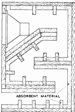
FIG. A/6. Typical acoustic labyrinth.
