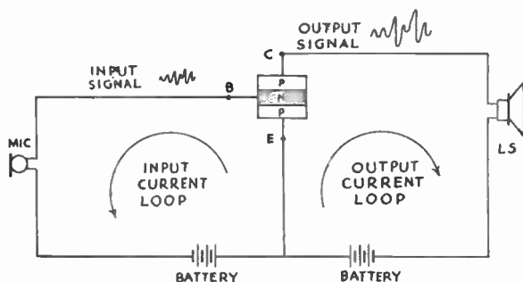
FIG. T/12. The transistor as an amplifier.
