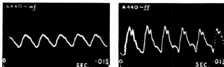
FIG. H/3. Oscillogram showing increase in harmonics when piano note is played loudly.
