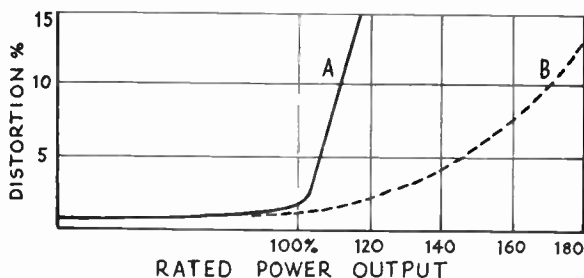
FIG. O/4. Amplifiers with different overload characteristics.
