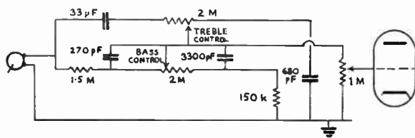
FIG. P/6. Input circuit for crystal or ceramic pickup, giving bass and treble boost and cut with overall volume control.
