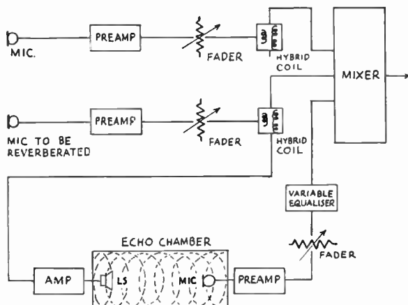
FIG. E/3A. Block diagram of recording channel with echo chamber.
