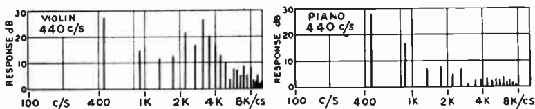
FIG. S/4. Sound spectrum or harmonic analysis of violin and piano tones.
