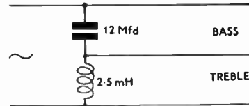
N.W.4. Quarter Section, Series
