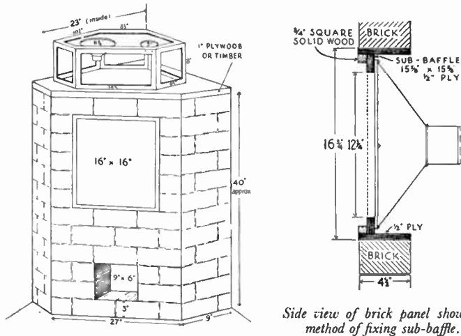
FIG. B/3. Brick corner enclosure, 9 cu.ft., used with no interior lining or absorbers.
