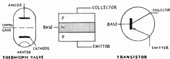
FIG. T/11. Valve and Transistor symbols. Courtesy Siemens Edison Swan Ltd.
