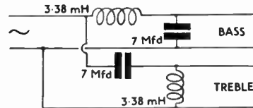
N.W.6. Half Section, Parallel
