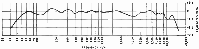
FIG. F/9A. Overall frequency response of microphone, amplifier and programme meter for sound source on microphone axis.
