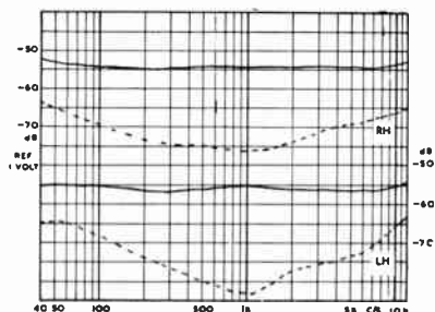
FIG. C/3. Good separation producing clean results, with full stereophonic "spread".
