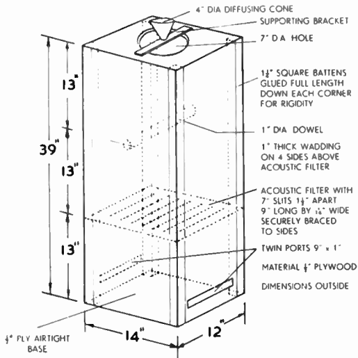
FIG. C/6. Plywood column (with solid wood corners) for 8" unit. Weight 30 lb. approx. Internal volume 3 cu.-ft. approx. The dowel must be tightly wedged between the two panels to control resonance.
