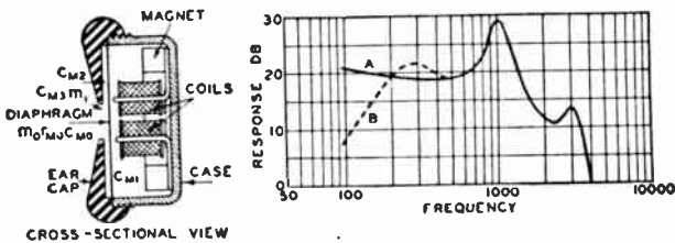
FIG. E/1. Diagram and response curve of magnetic earphone, taken from Olson's Elements of Acoustical Engineering .
