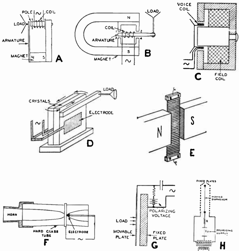
FIG. L/5. Driving Systems.
