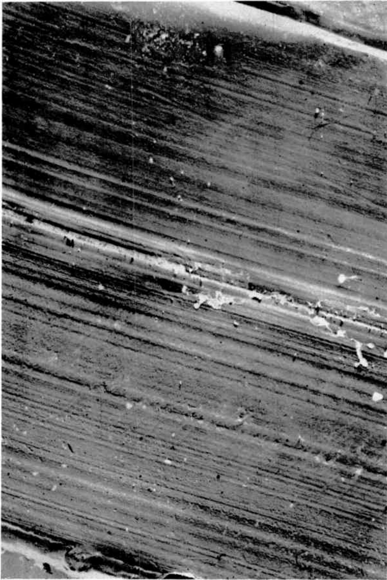
FIG. E/6A. Part of unplayed microgroove as revealed by Electron Microscope. Side view. Mag. 3,000x.
