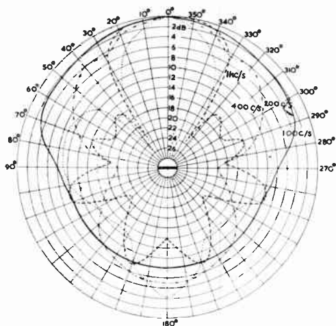
FIG. P/8A. Polar diagram of line source loudspeaker at 100, 200, 400 and 1,000 c/s.
