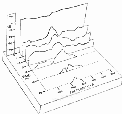
FIG. D/4. Interrupted tone test of loudspeaker. The rear portion represents the steady state response, and the others indicate different resonances which show up at intervals up to 40 milliseconds after termination of signal.
