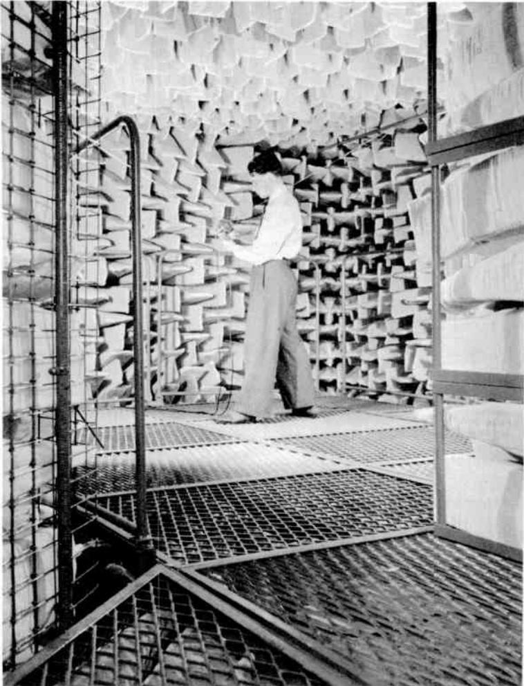
FIG. F/5. G.P.O. dead room.
