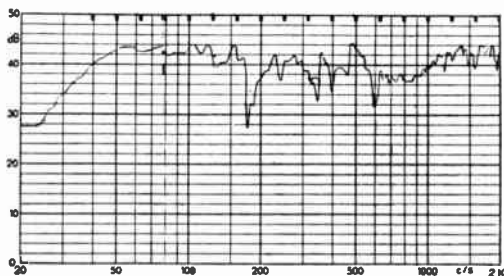
FIG. B/2. Response of 8" unit in 9 cu.ft. corner brick enclosure. Cone resonance 52 c/s. Input 1 watt.
