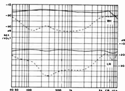
FIG. C/2. Typical response curves and separation between channels of crystal pickup.
