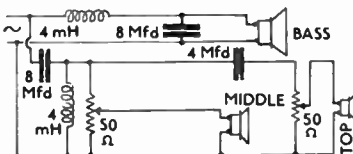
N.W.9. Half Section, 3-speaker circuit. Crossover at 800 and 5,000 c/s.
