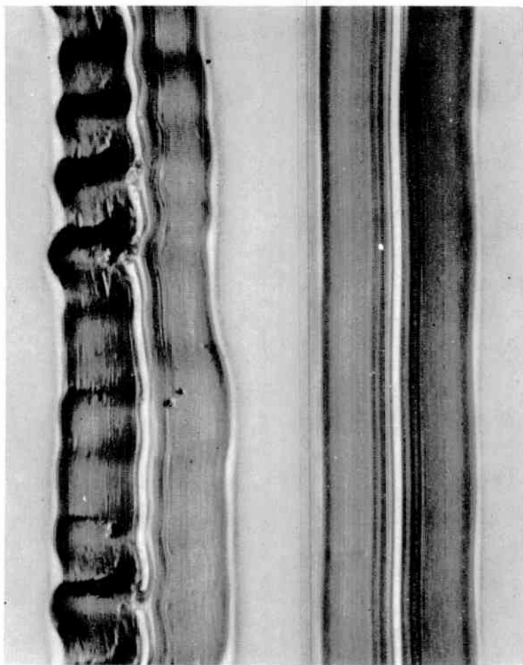
FIG. R/17. Heavily modulated groove after 165 playings showing slight signs of damage. Mag. 300x.
