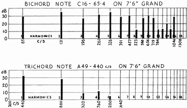
FIG. H/1. Harmonic analysis of two piano notes, showing high rate of overtones in bass compared with treble.
