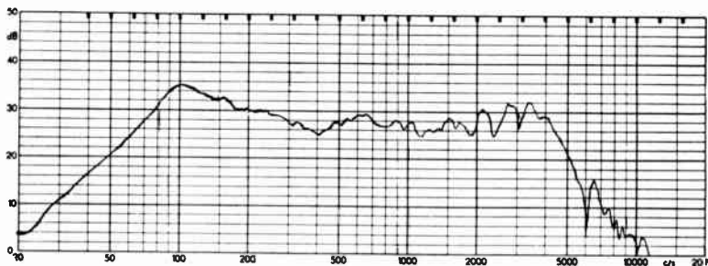
FIG. L/7. Axial response of 1930 model. Bass resonance 90 c/s.
