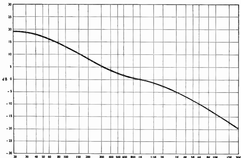
FIG. R/15. Standard replay characteristic for microgroove records in U.S.A. and Great Britain (R.I.A.A. and B.S.S. 1928/1955).
