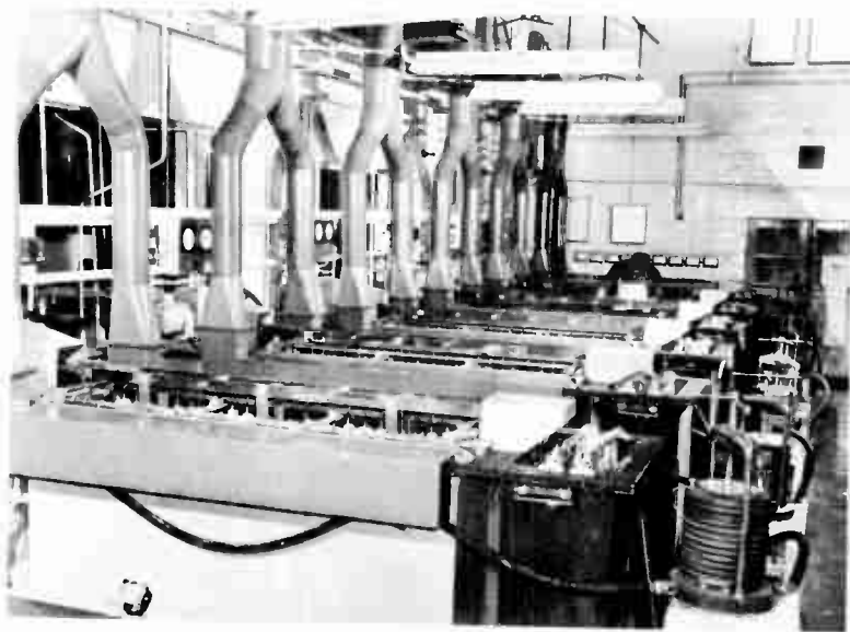
FIG. R/12. High speed nickel plating vats producing solid nickel stampers.
