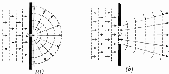
FIG. D/6. Sound waves passing through slot. (a) Width of slot less than wavelength. (b) Reverse order.
