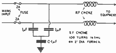
FIG. S/13. Circuit for reducing mains-borne interference with radio reception.
