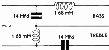
N.W.5. Half Section, Series
