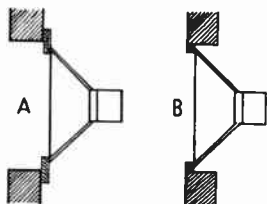
FIG. C/1A. To avoid cavity resonance use arrangement B.
