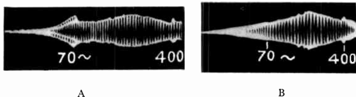
FIG. F/7. Oscillograms of free-field response from same cone and coil assembly. Input 1 watt. 8" unit. A With 8,000 oersted magnet. B With 13,000 oersted magnet.
