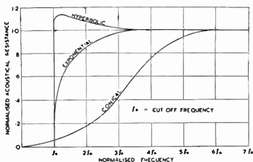
FIG. H/5. Acoustic resistance at horn throat for various flare shapes.
