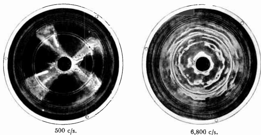
FIG. B/1. Illustrations of cone breakup.
