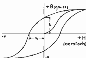
FIG. C/5. Typical magnetisation or BH curve.
