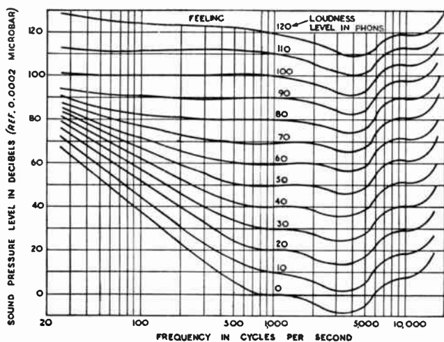
FIG. F/2. Equal loudness contours for pure tones. After Fletcher and Munson.
