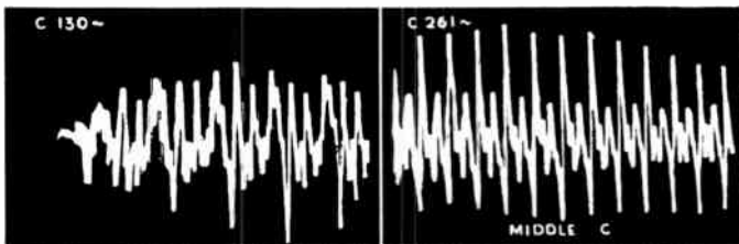
FIG. H/2. Oscillogram showing difference in harmonics between two piano notes only one octave apart.
