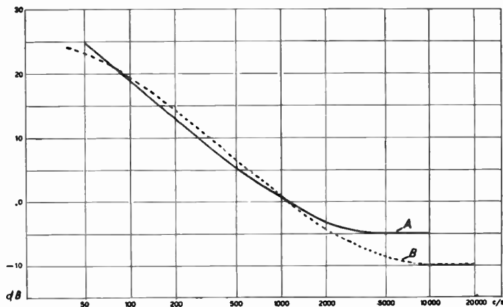
FIG. T/3. Standard replay characteristics for 7½"/sec tapes A—C.C.I.R. (British) B—N.A.R.T.B. (American)
