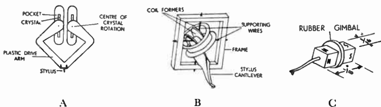
FIG. C/1. Cantilevers in stereo pickups.
