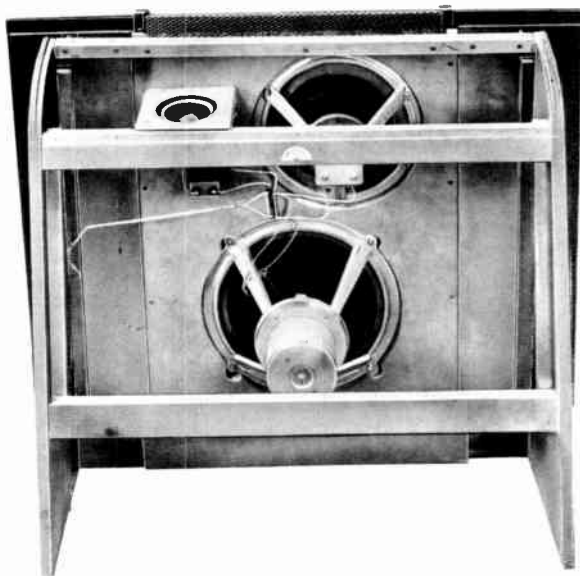
FIG. M/5. Two loudspeakers, 12" and 10", in parallel for improved LF output due to mutual radiation impedance.
