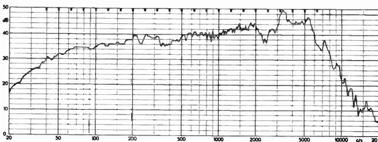
FIG. L/8. Axial response of modern 10" speaker. Bass resonance 35 c/s.
