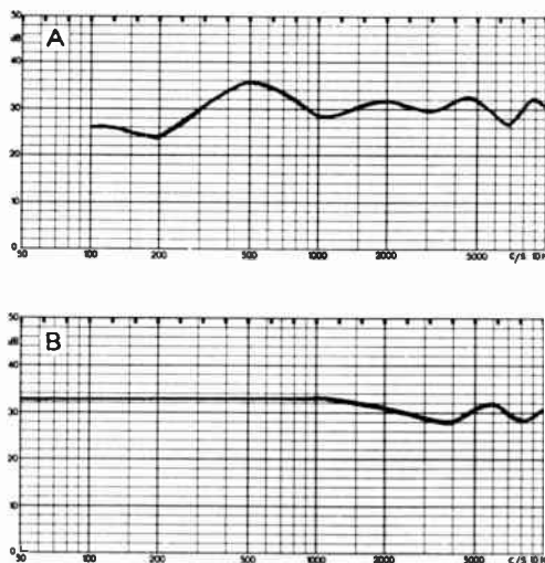
FIG. E/2. Typical response curves of earphones. A = crystal. B = moving coil.
