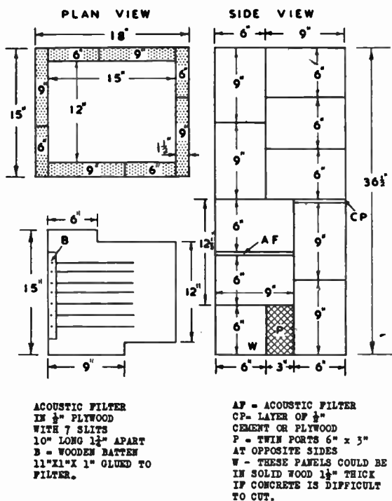
FIG. C/8. Concrete column, 4 cu.ft., using slabs 9" x 6" x \frac{1}{2} " and suitable for 8" and 10" units.
